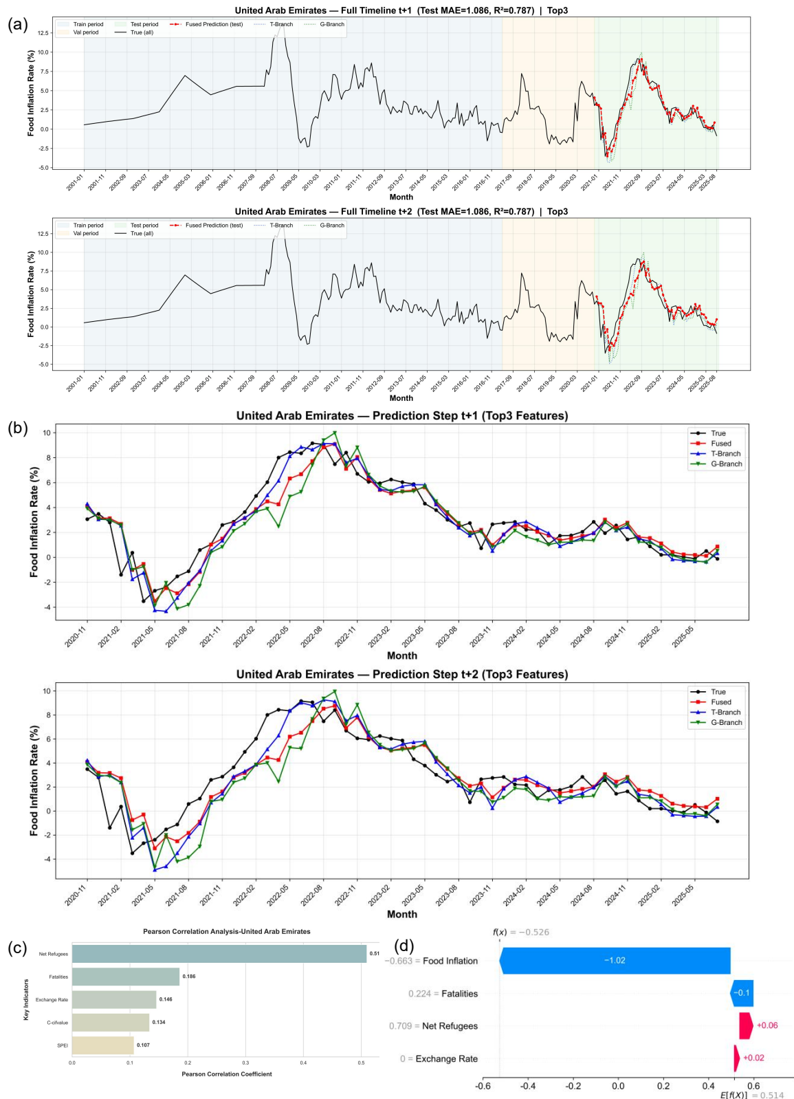
Multidimensional Evaluation and Attribution Analysis of Food Inflation Forecast in United Arab Emirates. (a) Overview of the total cycle prediction and fitting, (b) Multi-step Short-Term Forecast Comparison Chart, (c) Pearson correlation analysis of macroeconomic drivers, (d) SHAP-based explanation of feature contributions for a specific prediction instance.
